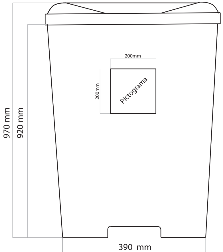
Vista Frontal
